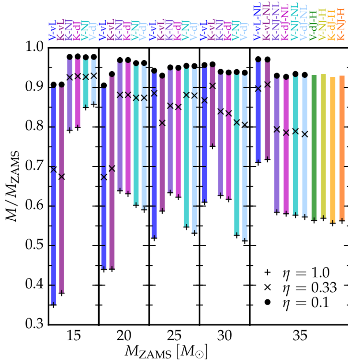
Fig. 1. Uncertainty in the mapping between M_{\text{ZAMS}} and the relative final mass M/M_{\text{ZAMS}} due to wind mass loss. Each colored bar corresponds to a specific wind algorithm combination defined in Table 2. The pluses, crosses, and circles correspond to \eta = 1.0, 0.33, 0.1 , respectively. We employ the vertical bars to emphasize the spread. The uncertainty in wind mass loss limits the predictive power of stellar evolution studies for the final mass of stars of given initial mass. Only models with M_{\text{ZAMS}} = 35 M_{\odot} and wind efficiency \eta = 1 reach the WR stage (cf. Table 4 and Sect. 3.4). They are shown in the rightmost panel and we list the WR mass loss algorithm only for them. The maximum relative mass for the four algorithm combinations using the H WR mass loss algorithm in the rightmost panel are the results obtained using the corresponding hot and cool mass loss combination with \eta = 0.1 (not reaching the WR phase).
