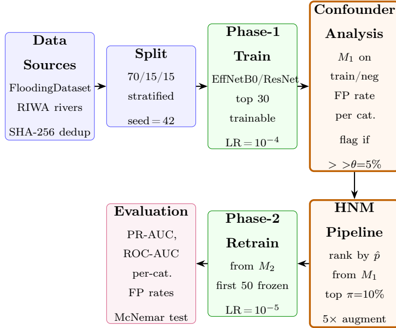
Figure 1: End-to-end methodology pipeline. Blue boxes: data preparation stages; green boxes: training stages; orange boxes (bold border): Phase-1 HNM novel contribution (??); purple box: evaluation. Data flows left-to-right in the top row; the HNM pipeline mines difficulty-ranked candidates from M_1 and retrains from M_2 .
