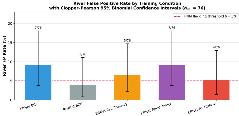
Figure 5: River false positive rate across all training conditions with Clopper–Pearson 95 % binomial confidence intervals ( N_{river}=76 in all conditions). The dashed horizontal line marks the Phase-1 HNM flagging threshold \theta=5\% . Wide CI overlap confirms that no pairwise difference is statistically significant at the available sample size. Annotated fractions show raw FP counts. Figure generated by scripts/plot_confounder_fp.py .
