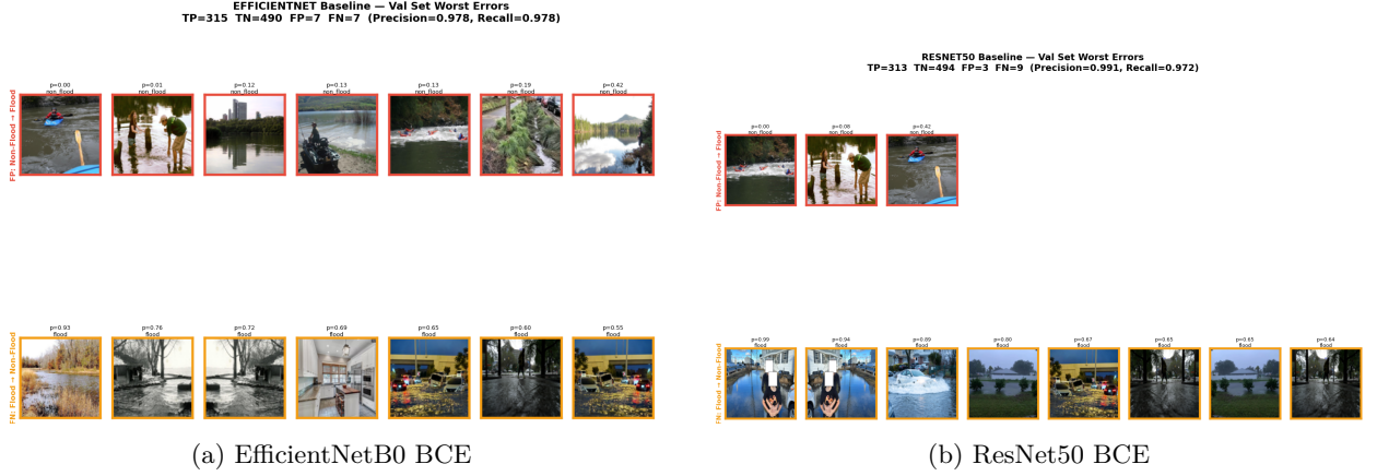
Figure 2: Worst false positives (red border, top rows) and false negatives (orange border, bottom rows) at \tau=0.5 (val set, seed 42). EfficientNetB0 FPs are visually ambiguous river scenes that share water texture with flood images. ResNet50 FNs include many prototypical flood scenes, indicating systematic rather than boundary-driven failure.
