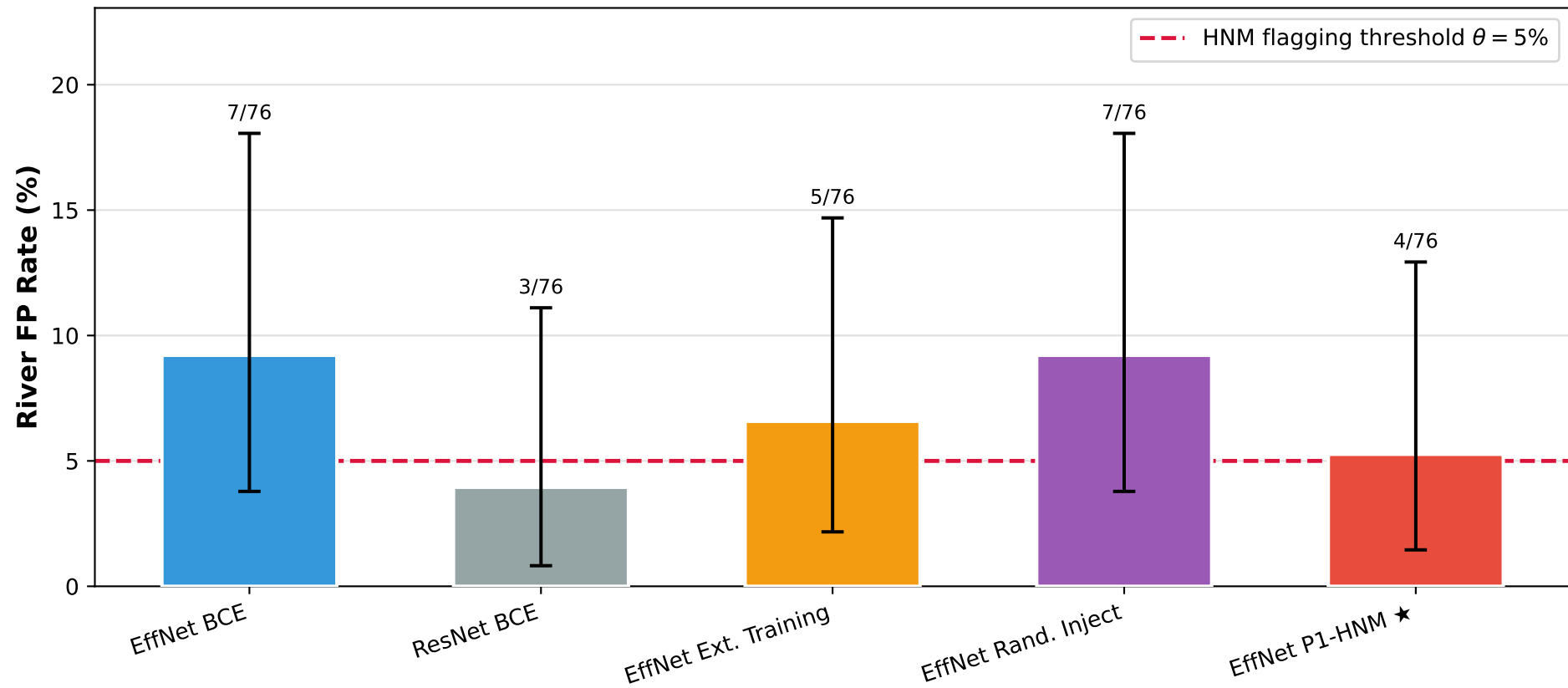
River False Positive Rate by Training Condition with Clopper-Pearson 95% Binomial Confidence Intervals ( N_{\text{val}} = 76 )
