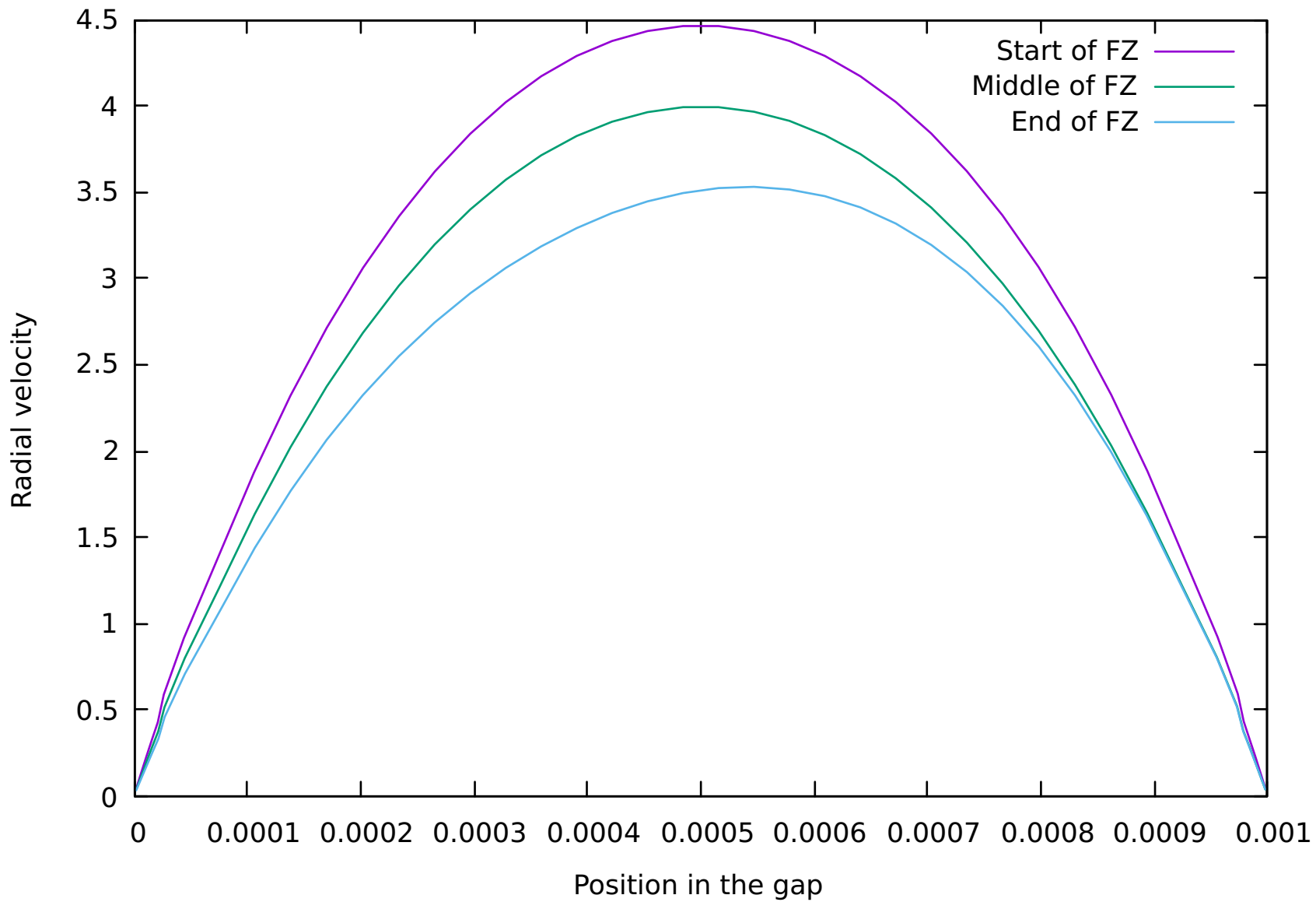
Radial velocity
