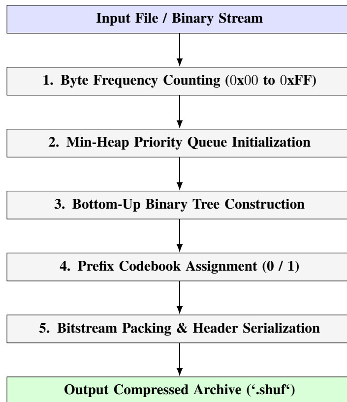
Figure 1: High-Level Flowchart of Huffman Compression Pipeline
