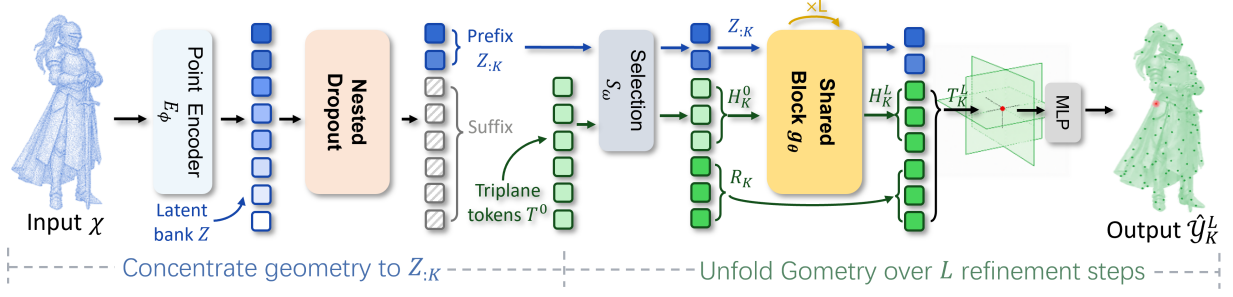
Figure 1 Overview of ZipTok3D. Nested dropout concentrates geometry into a reconstructive prefix Z_{:K} , while the parameter-shared block progressively unfolds it into triplane features over L refinement steps. Blue and green denote latent and triplane tokens, respectively; hatched tokens indicate the masked suffix.
