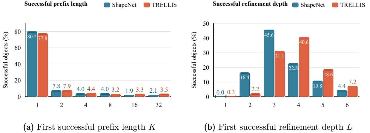
Figure C Adaptive-budget distributions under the token-first all-metric search. The left panel shows the first successful prefix length K and the right panel the first successful refinement depth L ; percentages are normalized within the successful subset of each dataset.
