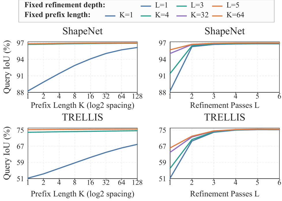
Figure 3 Effect of prefix length K and refinement depth L on query IoU for ShapeNet (top) and TRELIS (bottom). The plots vary K at fixed L (left) and L at fixed K (right).
