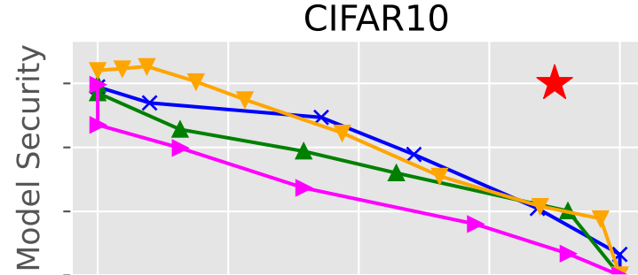
AlexNet
