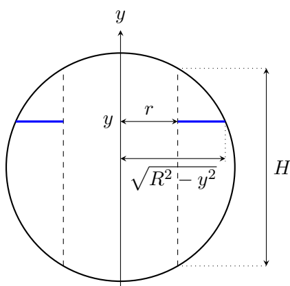
Figure 3.6: A meridian section of the drilled sphere. The blue segments rotate into one annulus. At each height use the outer radius at that same height and the fixed inner radius r .
