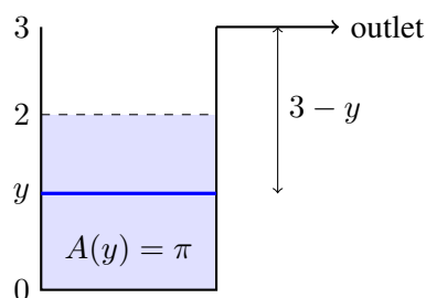
Figure 3.8: Use a horizontal fluid slice. Its cross-sectional area and its lift are different factors in the work integral. Heights are in metres.
