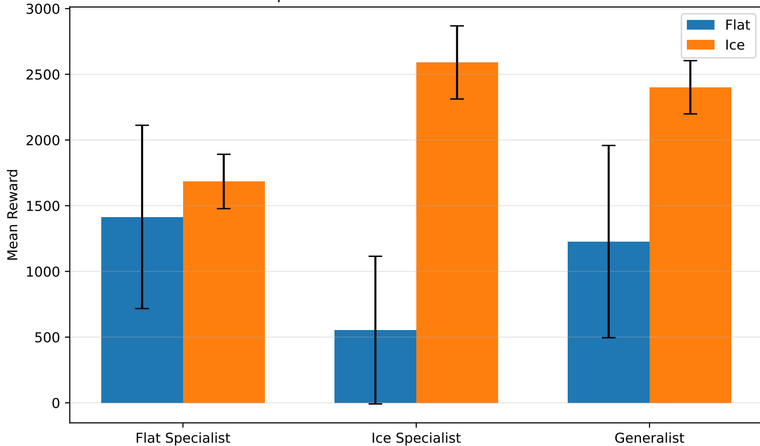
Specialist vs Generalist Performance
