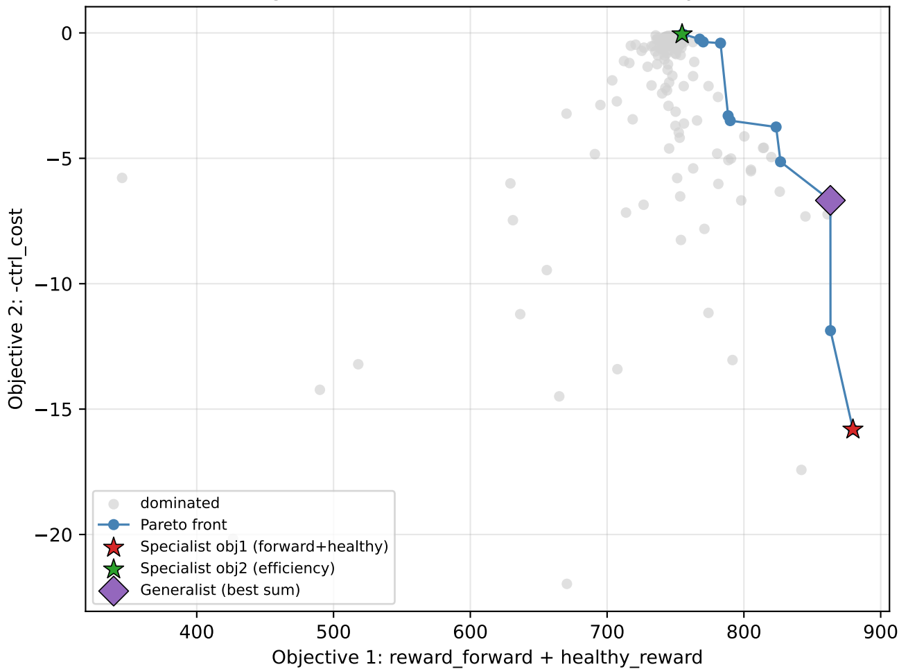
Challenge 3 — Final NSGA-II Pareto Front (hilly terrain)
