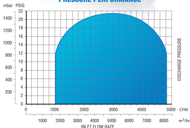
PRESSURE PERFORMANCE
