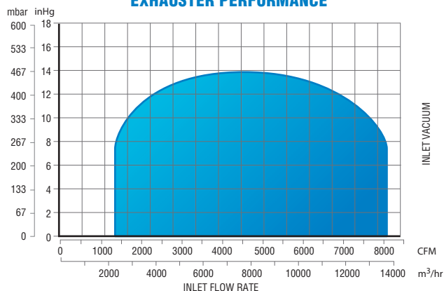
EXHAUSTER PERFORMANCE
