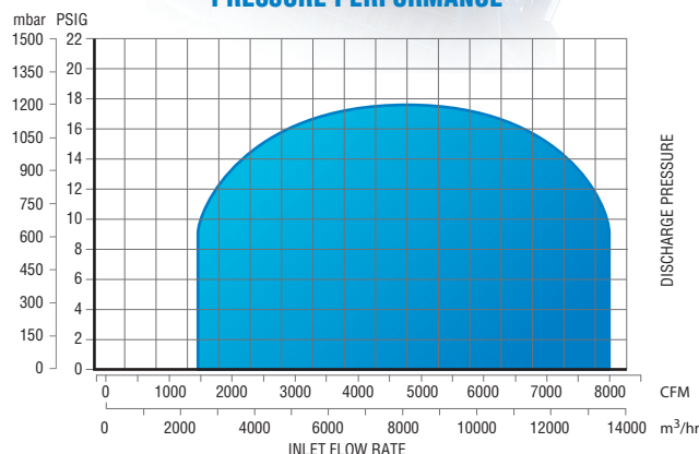
PRESSURE PERFORMANCE
