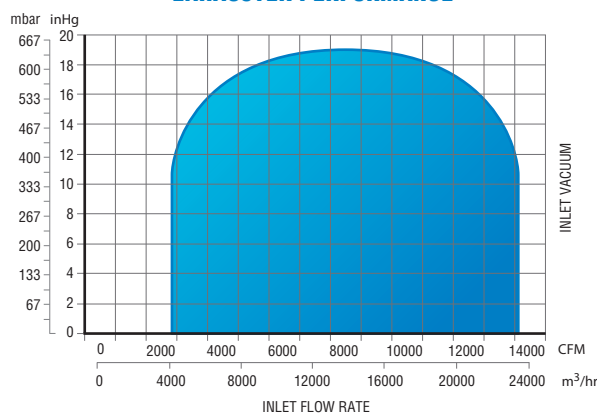
EXHAUSTER PERFORMANCE
