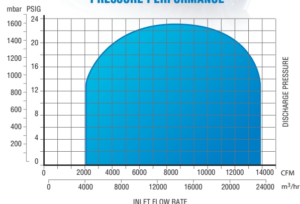
PRESSURE PERFORMANCE
