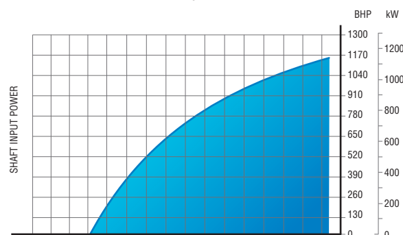
EXHAUSTER PERFORMANCE
