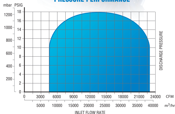
PRESSURE PERFORMANCE
