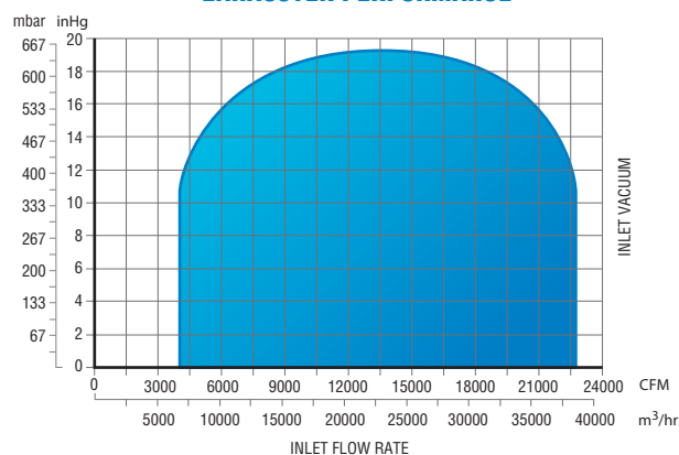
EXHAUSTER PERFORMANCE
