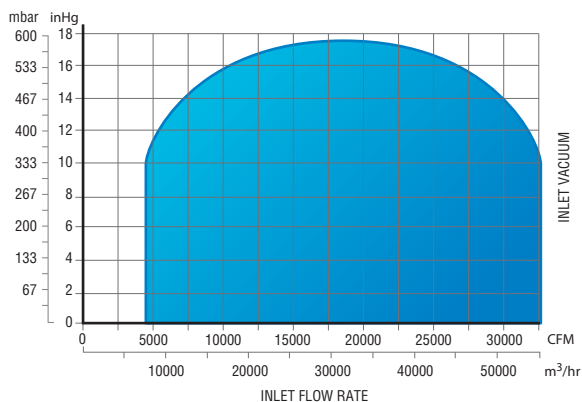
EXHAUSTER PERFORMANCE
