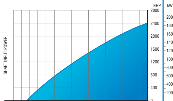
EXHAUSTER PERFORMANCE
