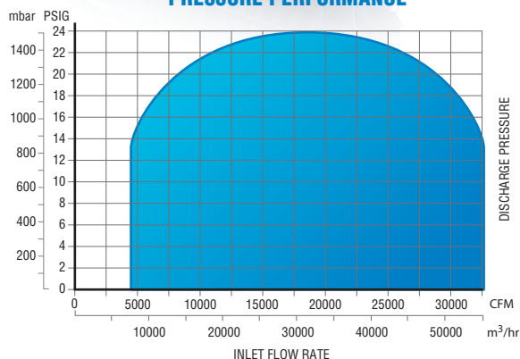
PRESSURE PERFORMANCE
