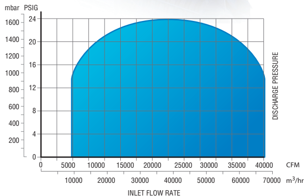
PRESSURE PERFORMANCE
