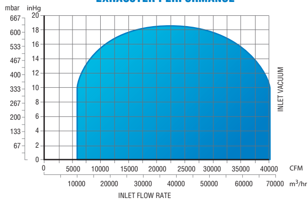
EXHAUSTER PERFORMANCE
