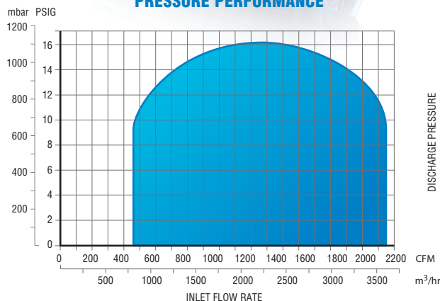
PRESSURE PERFORMANCE
