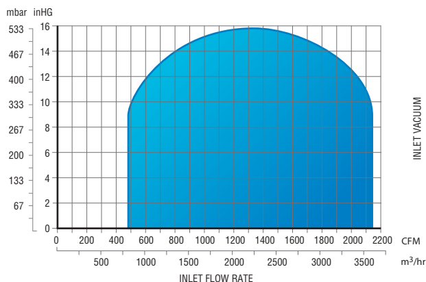
EXHAUSTER PERFORMANCE
