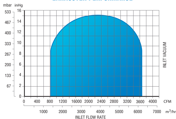
EXHAUSTER PERFORMANCE
