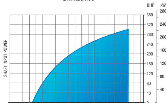
EXHAUSTER PERFORMANCE
