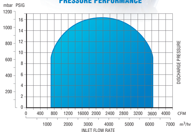
PRESSURE PERFORMANCE
