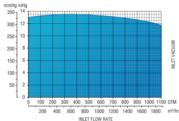
EXHAUSTER PERFORMANCE
