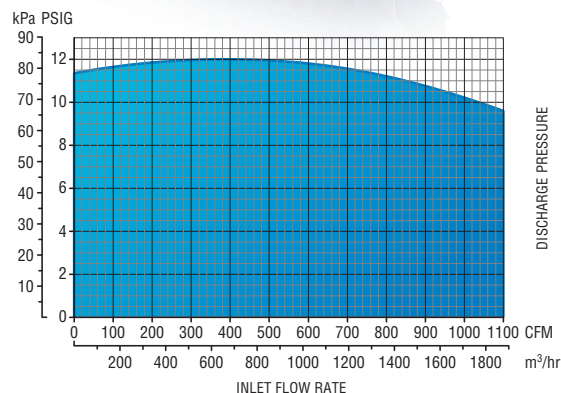
PRESSURE PERFORMANCE
