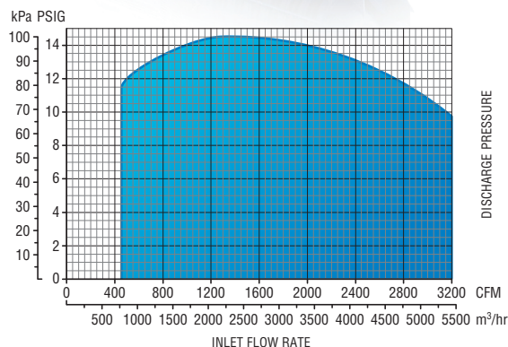
PRESSURE PERFORMANCE
