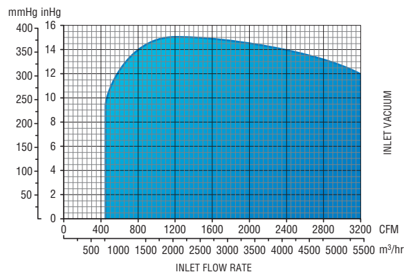
EXHAUSTER PERFORMANCE
