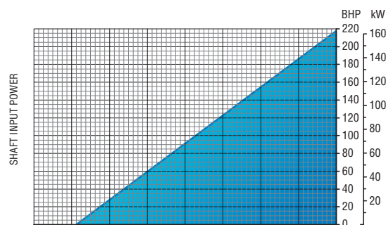
EXHAUSTER PERFORMANCE
