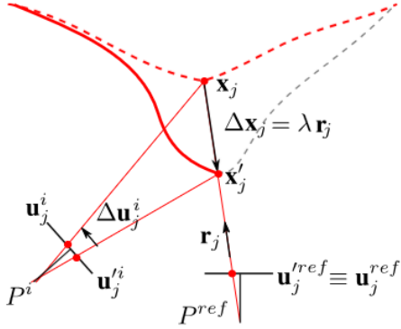
Figure 3: Geometry of our scene flow update. All updates to the base surface vertices are constrained along viewing rays of the reference camera.
