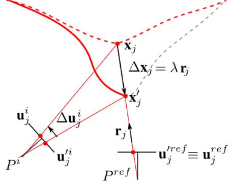
Figure 5: Geometry of our scene flow update. All updates to the base surface vertices are constrained along viewing rays of the reference camera.
