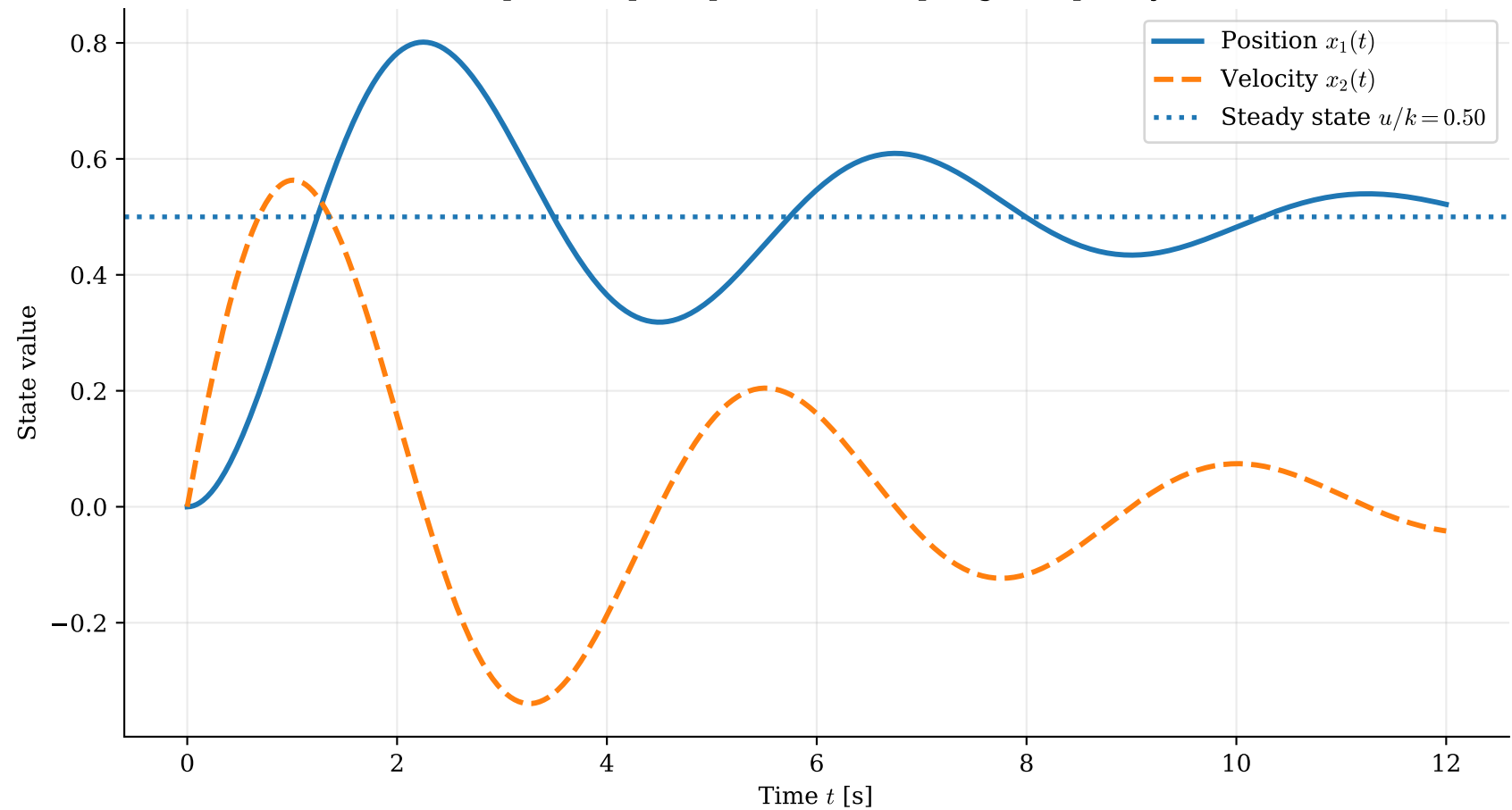
State-Space Step Response: Mass-Spring-Damper System
