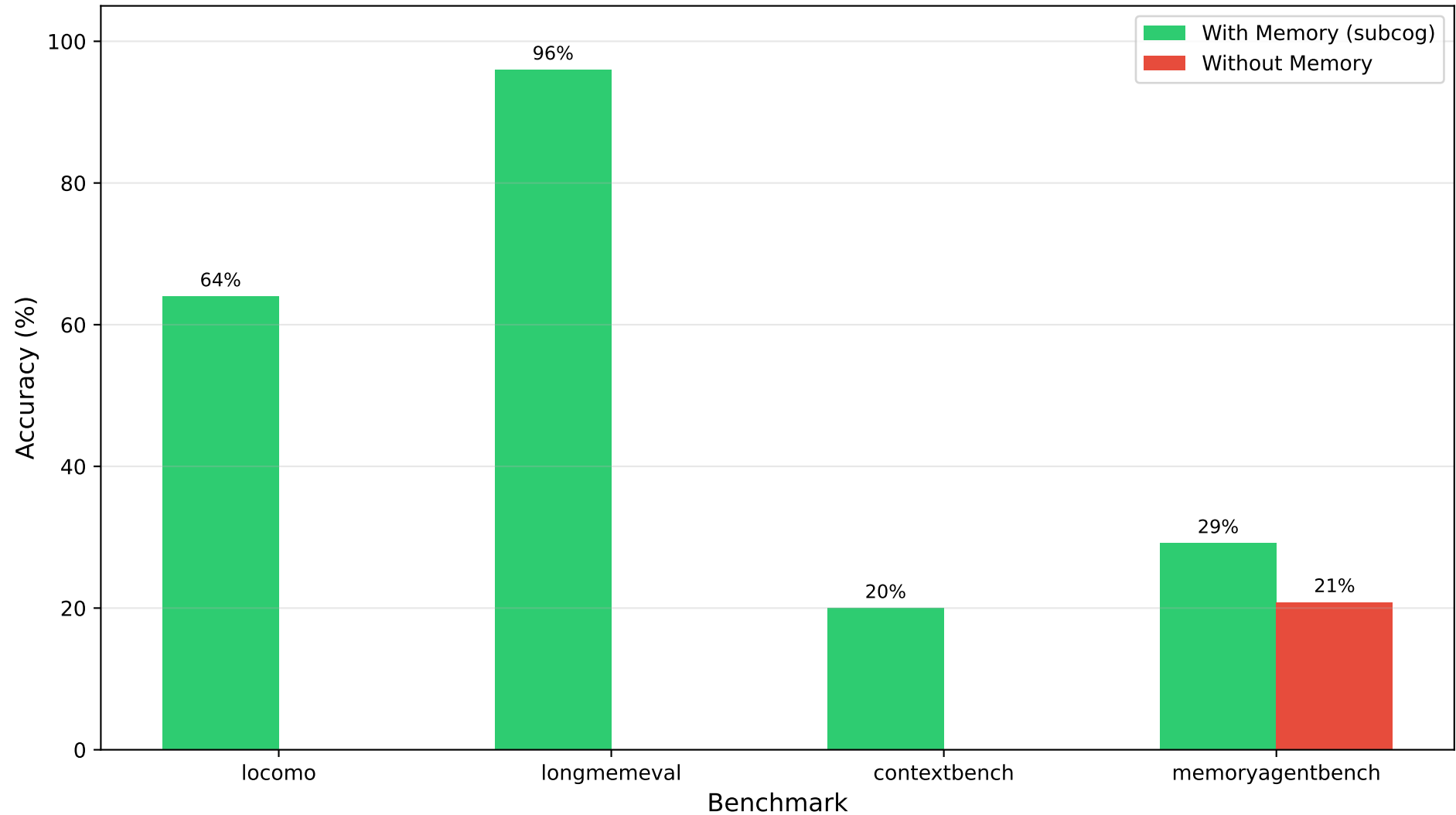
Memory System Benchmark Results (gpt-5.2, n=25)
