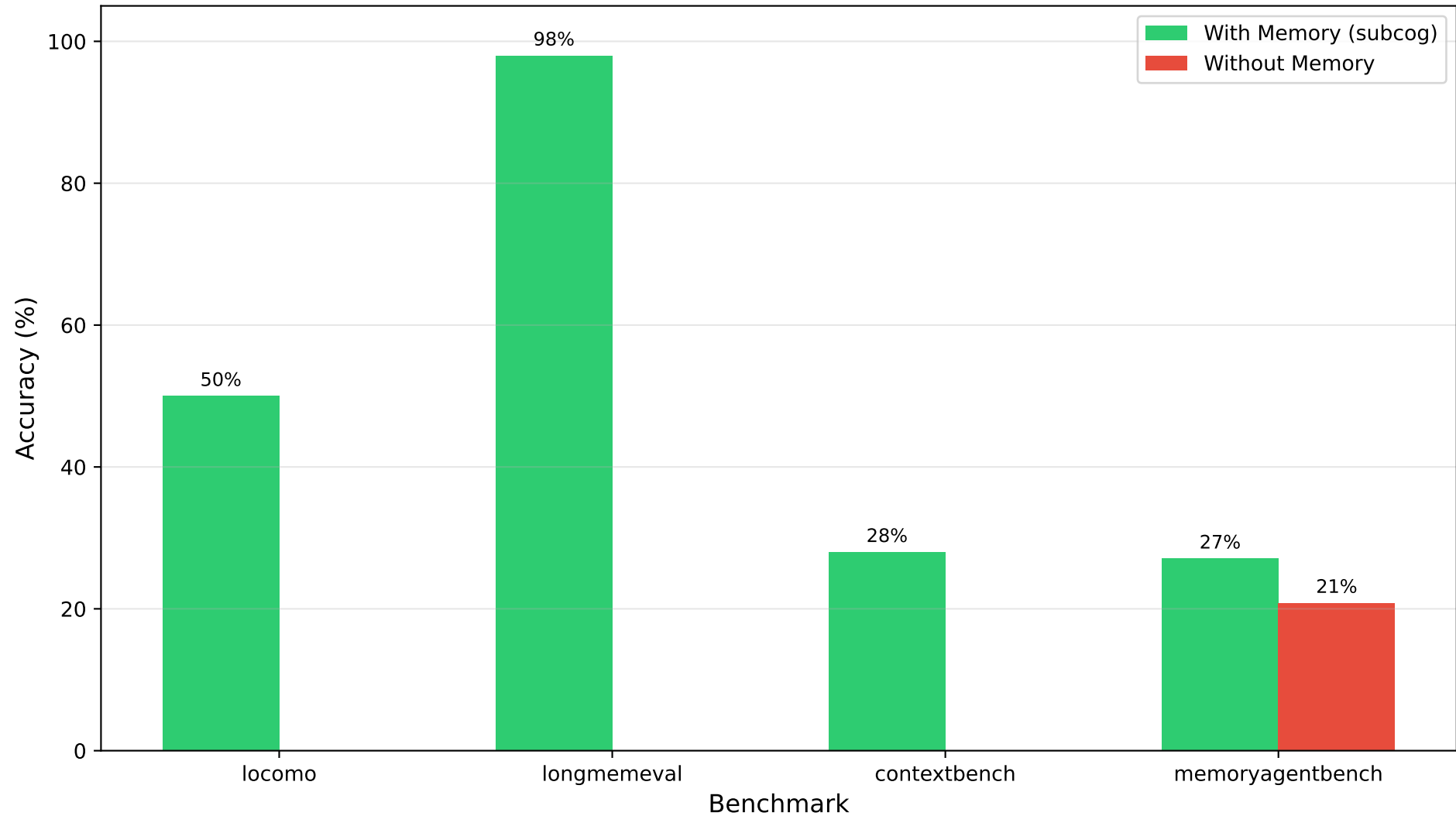
Memory System Benchmark Results (gpt-5.2, n=50)
