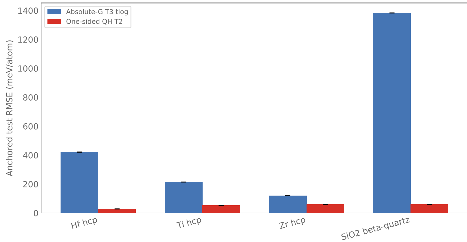
Single-sided QH thermal-shape diagnostic
