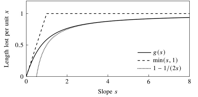
Fig. 2. The defect density g(s) = 1 + s - \sqrt{1 + s^2} , which is the length lost per unit of horizontal distance along a stretch of slope s , with the bounds (14) and (15). The loss is small for gentle slopes and approaches the full horizontal step for steep ones.
