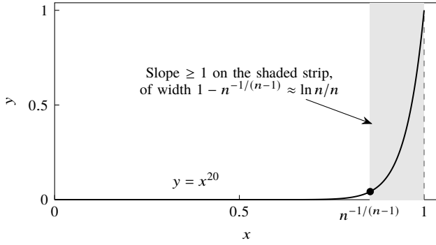
Fig. 6. Origin of the defect of x^n for n = 20 . The curve has slope at least 1 only on the shaded strip. There it climbs from height about 1/n (dot) to 1 while moving horizontally by about \ln n/n , and almost all of that horizontal movement is lost relative to the corner path.
