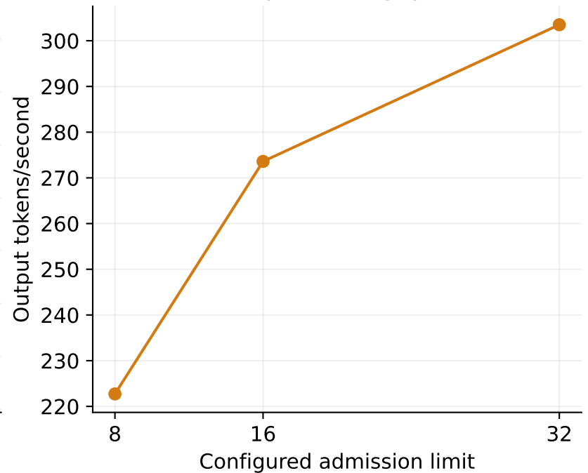
Output throughput
