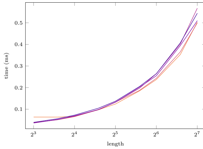
Figure 3: Average time to generate any trace of specific length using random walks. Each line corresponds to one of the models depicted above.
