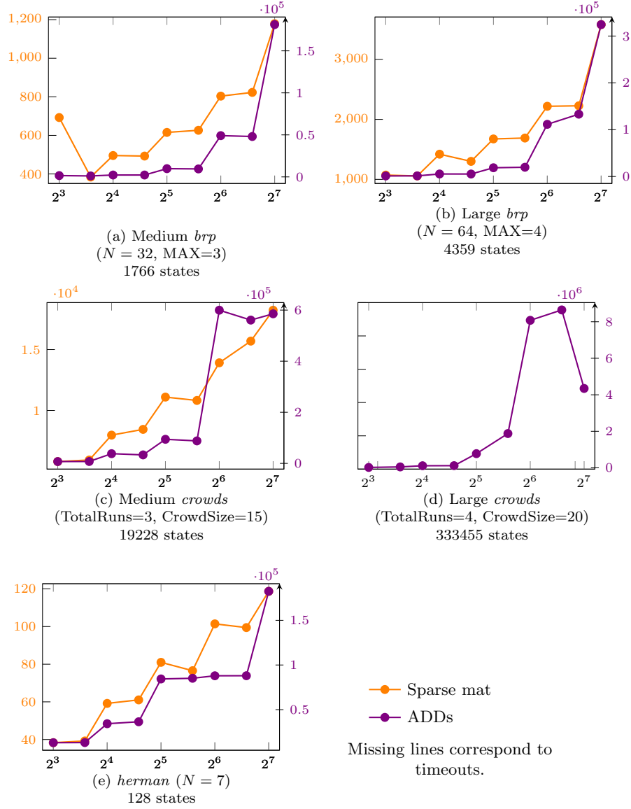
Figure 2: Precomputation time comparison across models and trace lengths. x-axis: Length, left (orange) y-axis : sparse matrix time (ms.), right (violet) y-axis : ADD time (ms.).
