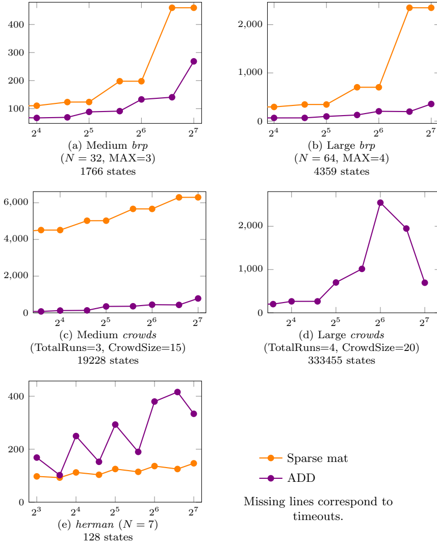
Figure 1: Maximum resident set size as reported by the system. x-axis: Length, y-axis: memory (mb).
