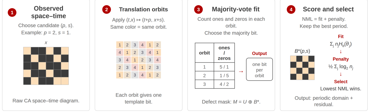
Figure 1: The Winnower pipeline on a small example. (1) The observed space-time U (time running downward). (2) A candidate (p, s) partitions cells into translation orbits: cells with the same number must be equal if the candidate is right. (3) A majority vote inside each orbit produces the minimum-Hamming domain template B^*(p, s) ; cells that lost their vote form the defect mask M = U \oplus B^* . (4) Each candidate is scored by fit (Bernoulli negative log-likelihood, NLL) plus a complexity penalty; the candidate with the lowest total (Bernoulli NML) wins.
