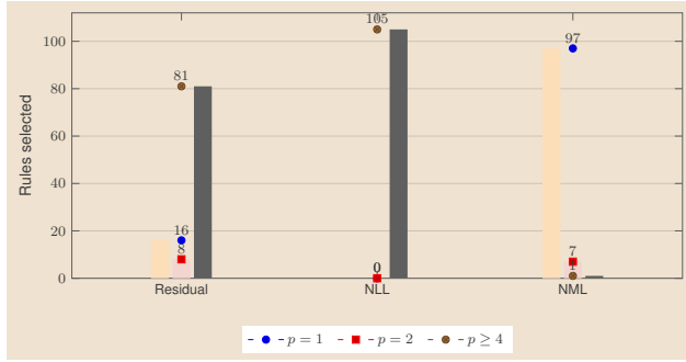
Figure 4: Selector ablation on the 105 non-degenerate Life-like rules at T = 100 (single seed). Bars count rules by the period each criterion selects. Raw defect-count minimization (the axis label Residual keeps the earlier draft name) and plain Bernoulli NLL are pulled toward the largest scanned period; Bernoulli NML concentrates selections at low period.
