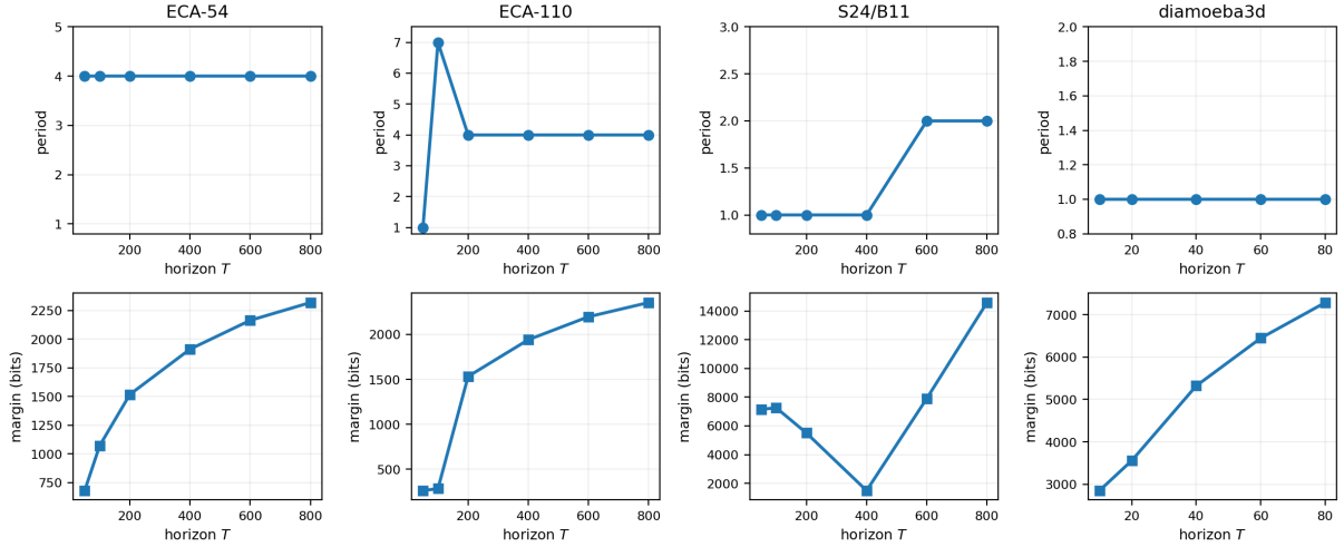
Figure 2: Representative stabilization patterns. The top row shows selected period versus horizon; the bottom row shows the winning margin in bits. The period either stabilizes immediately (ECA-54, diamoeba3d) or changes only a small number of times before locking (ECA-110, S24/B11).
