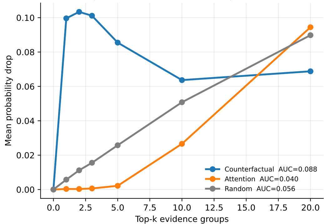
Comprehensiveness: remove top-k evidence
