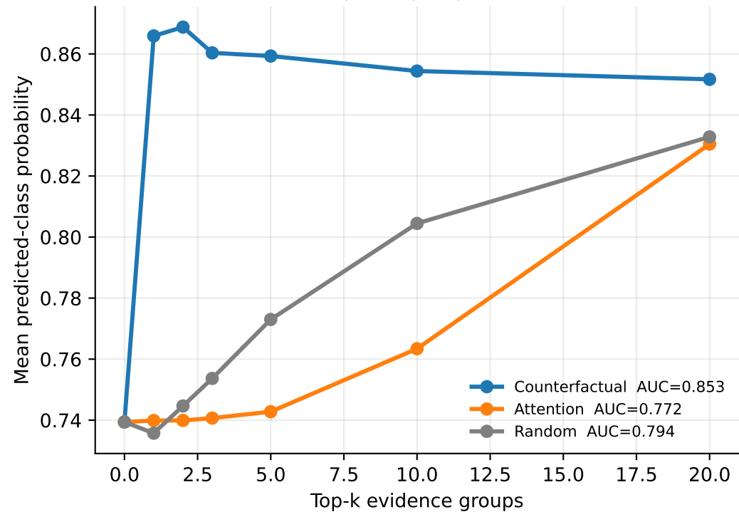
Sufficiency: keep top-k evidence
