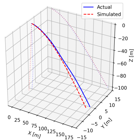
Figure 2: Actual vs. simulated ski jump trajectory
