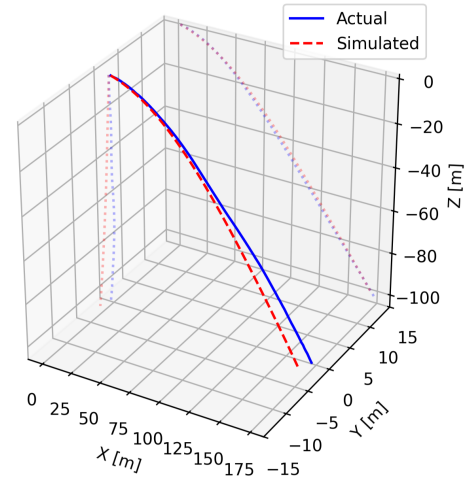
Figure 1: Actual vs. simulated ski jump trajectory
