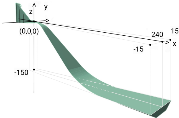
Figure 1: 3D model of Ski jump in Planica with added coordinates [8] [1]
