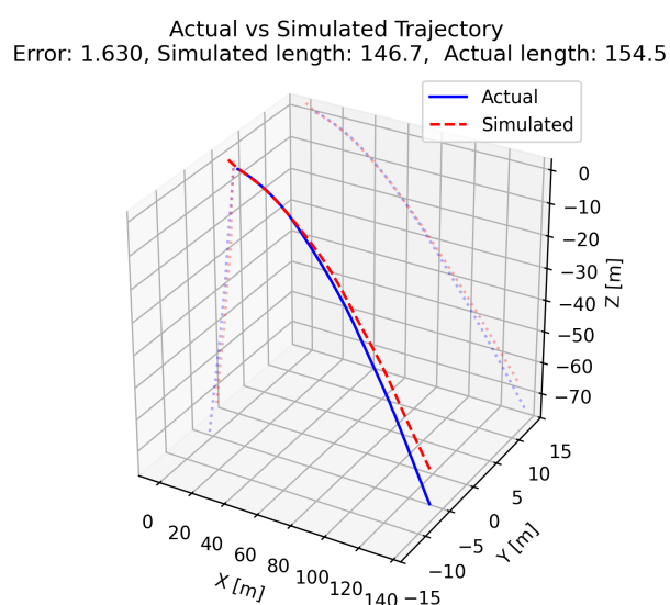
Figure 5: Actual vs. simulated ski jump trajectory
