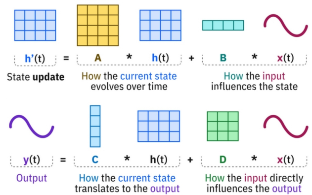
Figure 4: Schema of SSM matrices [3]
