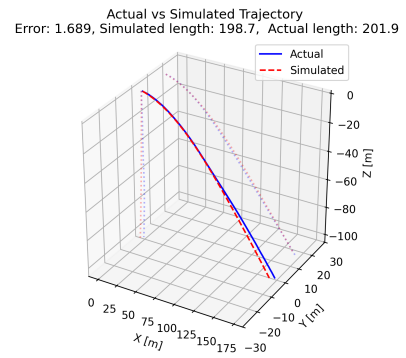
Figure 1: Actual vs. simulated ski jump trajectory
