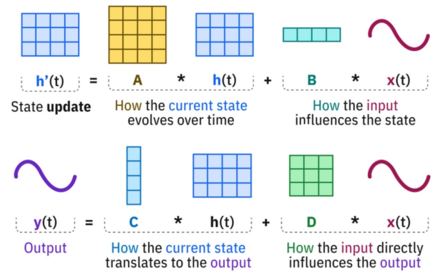
Figure 3: Schema of SSM matrices [3]
