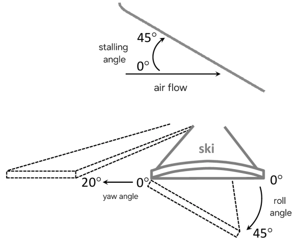
Figure 2: Different angles affecting the jump
