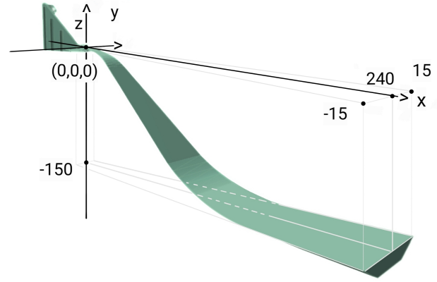
Figure 1: 3D model of Ski jump in Planica with added coordinates [1, 10].
