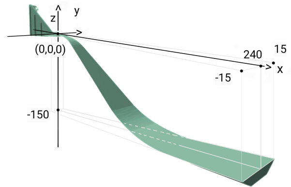
Figure 2: 3D model of Ski jump in Planica with added coordinates [12, 1]
