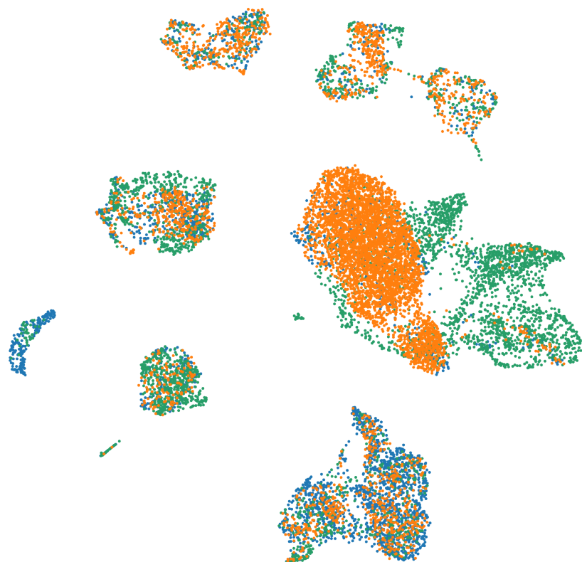
Sample — Harmony integrated
