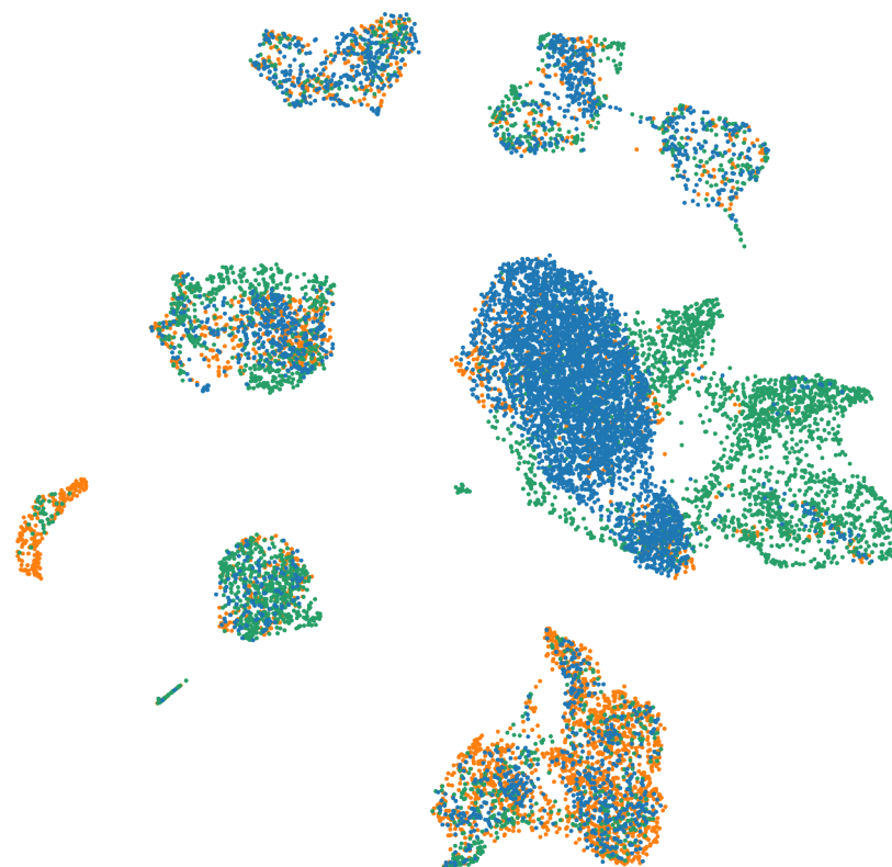
Subtype — Harmony integrated
