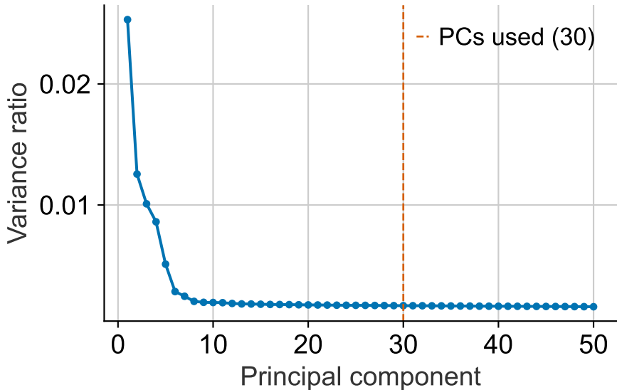
PCA scree plot
