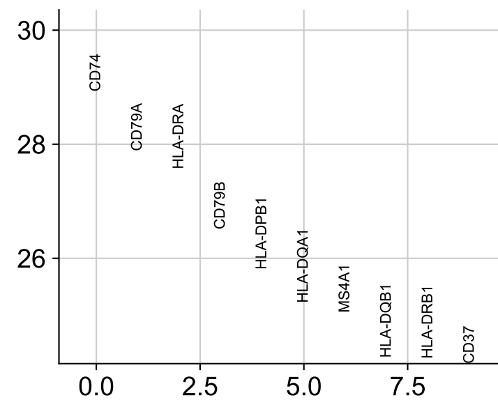
1 vs. rest
