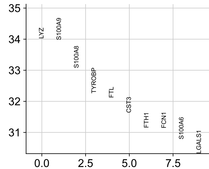
2 vs. rest
