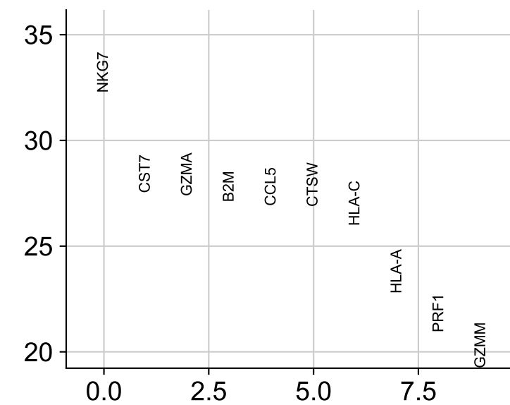
3 vs. rest
