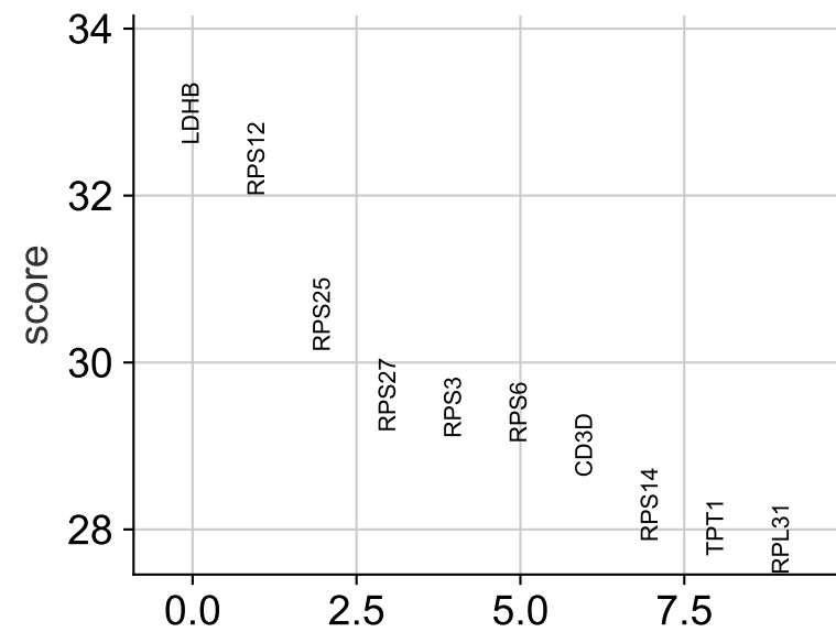
0 vs. rest
