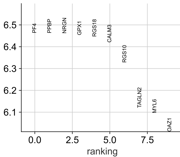
5 vs. rest
