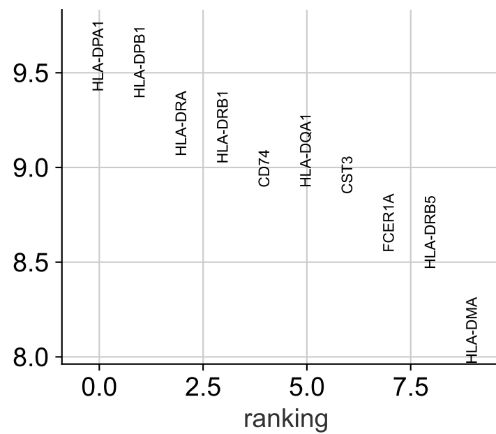
6 vs. rest
