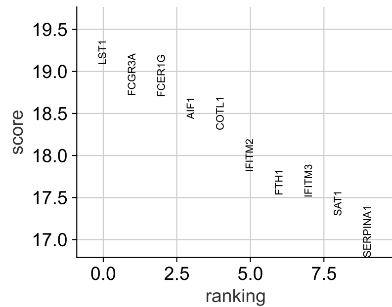
4 vs. rest
