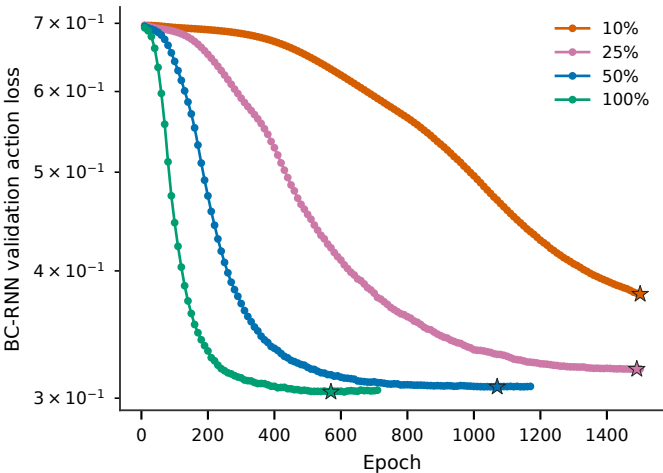
Data fraction: BC-RNN
