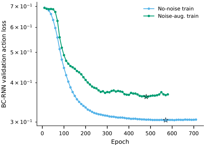
BC-RNN
