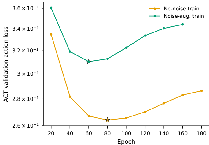
ACT
