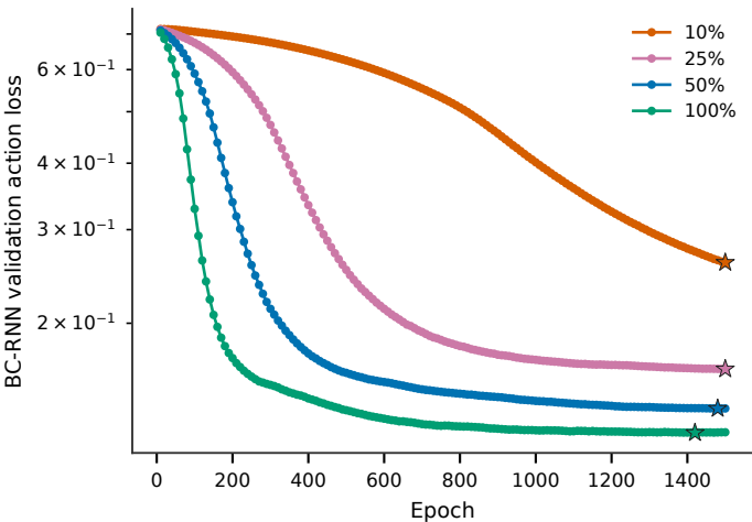
Fixed-axis data fraction: BC-RNN
