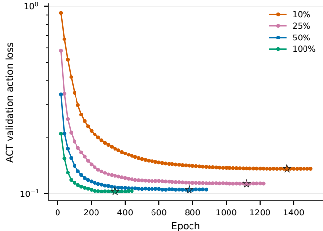
Fixed-axis data fraction: ACT
