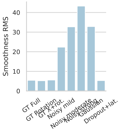
Trajectory roughness
