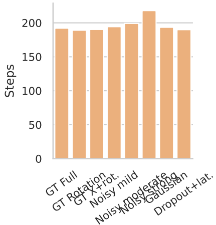
Completion length
