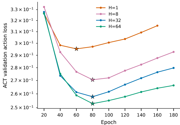
History horizon: ACT
