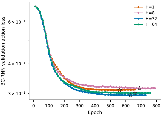
History horizon: BC-RNN
