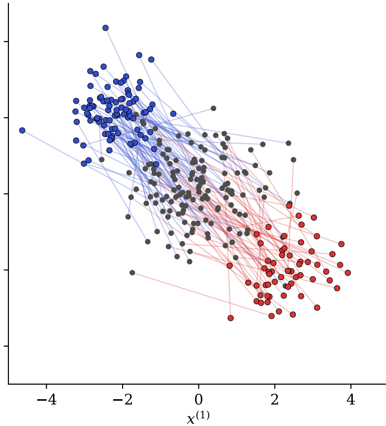
(b) Stage II: one-step generation x_1 = x_0 + v , v \sim \tilde{\pi}(v | x_0, 0) (no NN)
