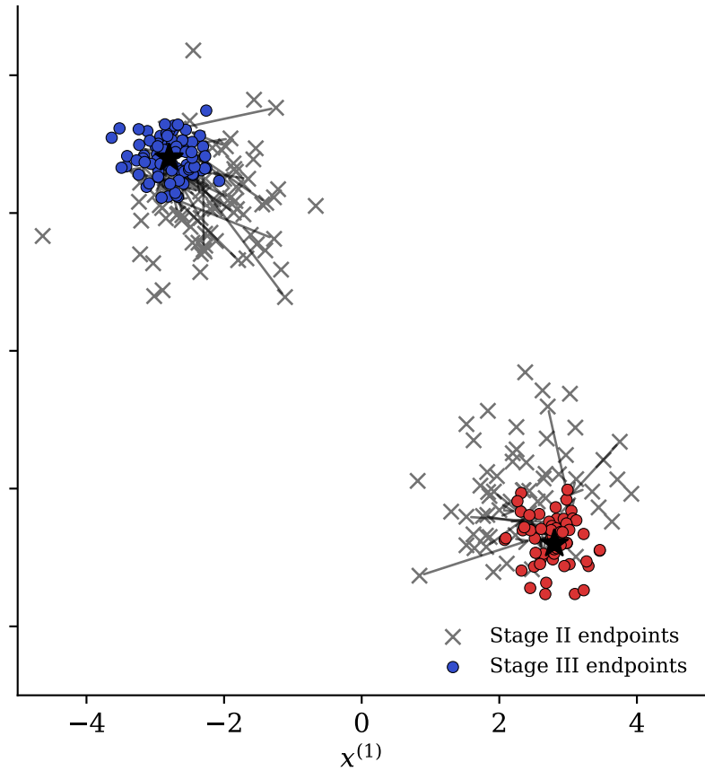
(c) Stage III: correction closes the small residual (Stage II \rightarrow \pi )
