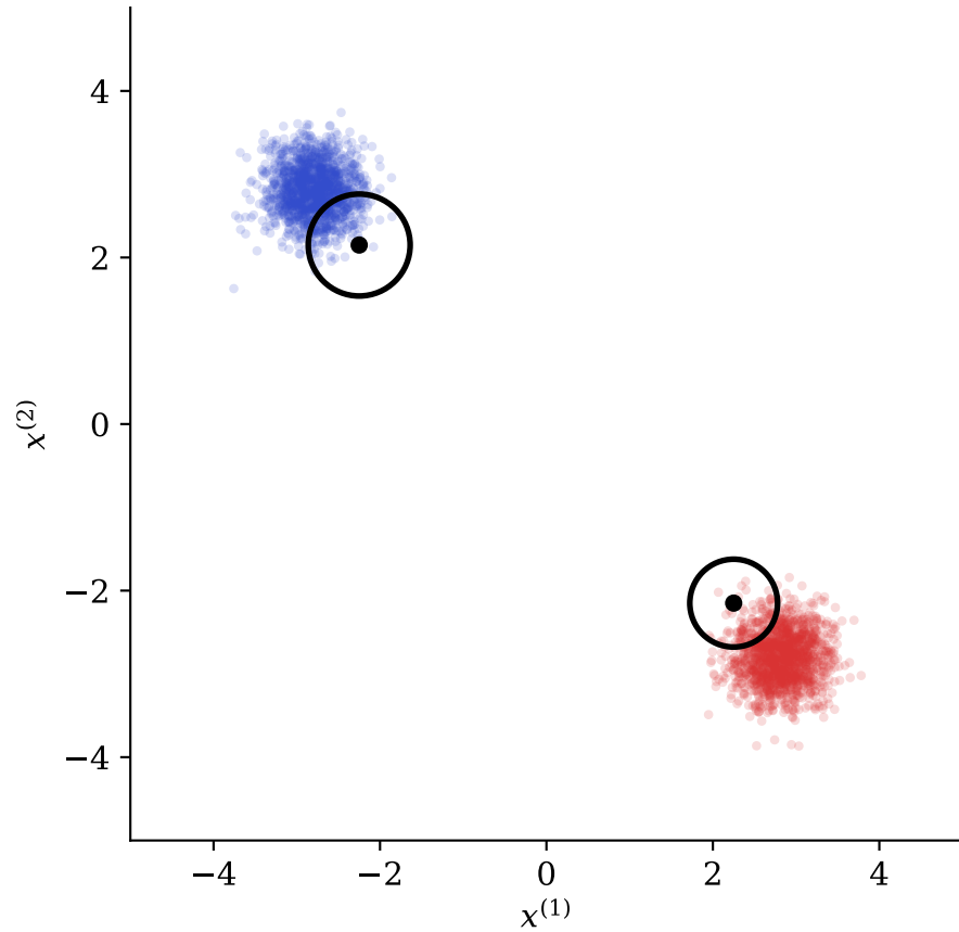
(a) Stage I: weighted coresets of \rho_1 K = 2 atoms (black), weights by circle size
