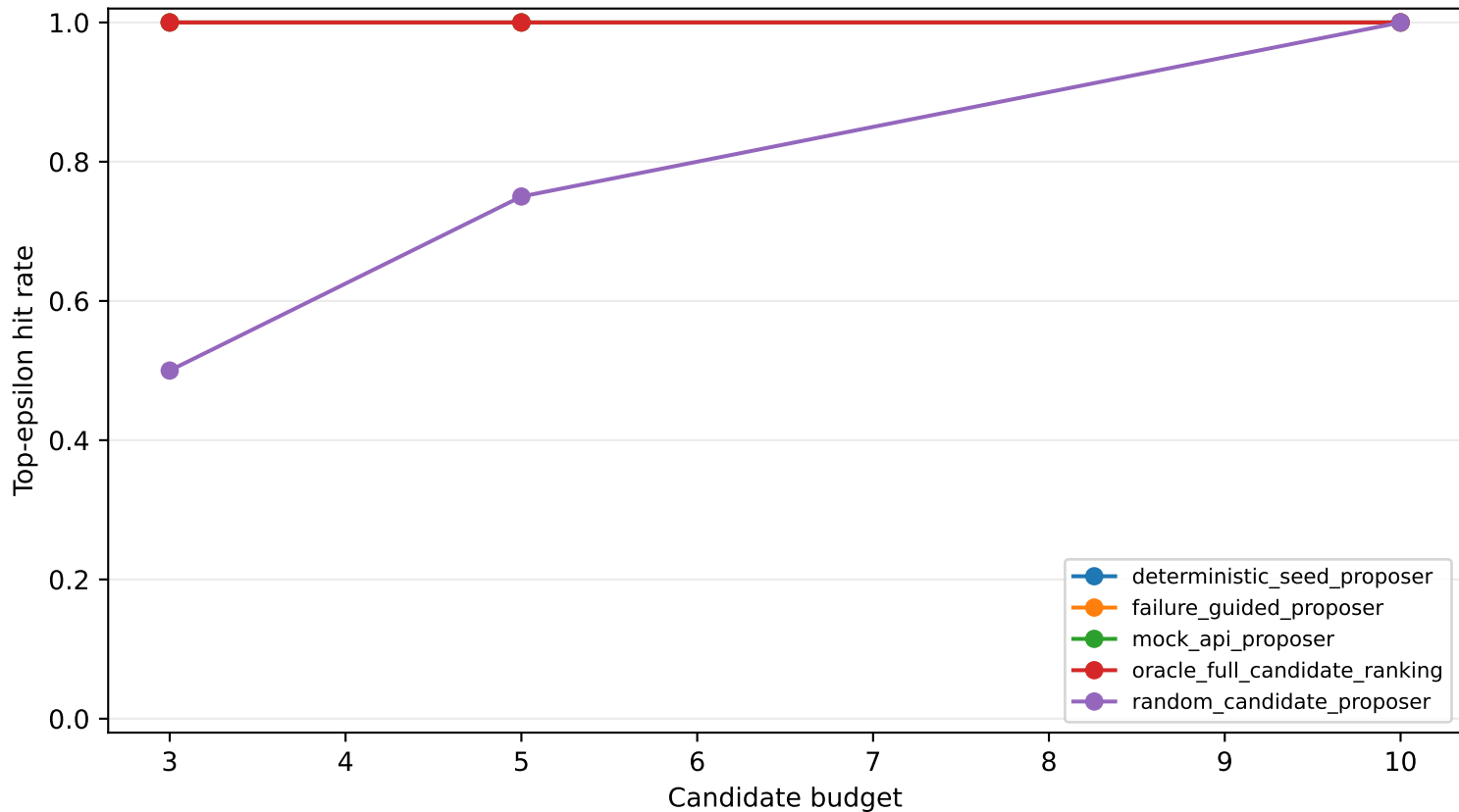
Bounded real-data execution by candidate budget
